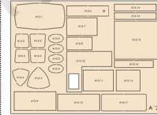
Ratio1:6 A12 Wooden block (wood color)18*13.5*0.2(1piece)
