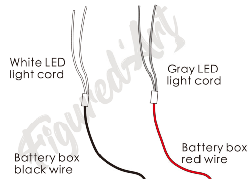
The black wire of the battery box and the white LED light wire, and the red wire and gray LED light wire of the battery box are connected together.
